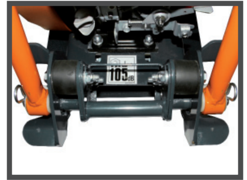
ANTI-VIBRATION HANDLE MOUNTS & REAR LIFTING HANDLE
